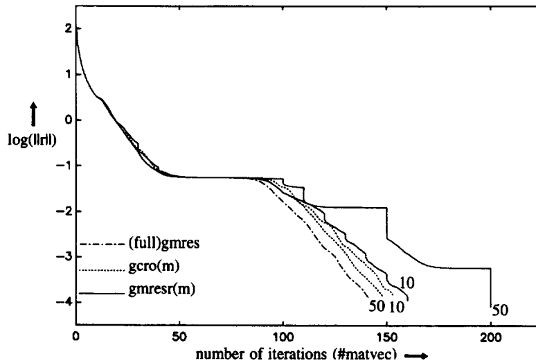
Fig. 14. Convergence vs. number of iterations for Problem 3.
