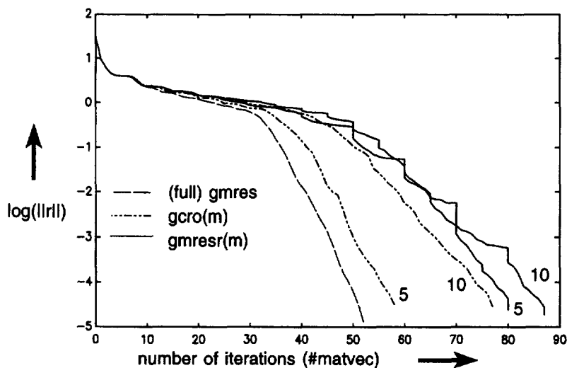
Fig. 12. Convergence vs. number of iterations for Problem 2.
