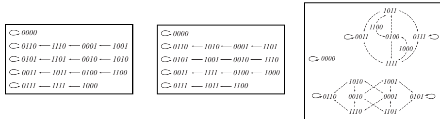
Fig. 0.1. Please note that the actual figure caption is omitted. This is the replacement for Figure 8.1. Also added: In rightmost phase space solid edges have probability 1, dashed edges have probability 1/2.
