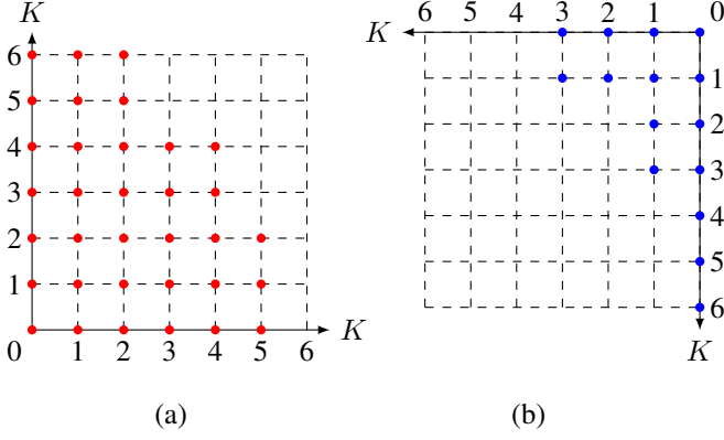
Fig. 1. The code C(\mathcal{S}, \mathcal{M}) in Example 3.4 is generated by the vectors \text{ev}_{\mathcal{S}}(M) where M is the set of monomials whose exponents correspond to points in (a). Its dual C(\mathcal{S}, \mathcal{M})^\perp is generated by the vectors \text{Res}_{\mathcal{S}}(M) where M is the set of monomials whose exponents correspond to points in (b).
