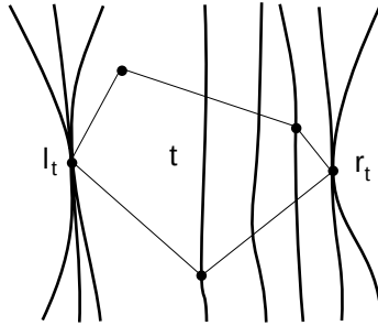
Figure 6.2.6. The tile t , the vertices l_t, r_t and the arcs which meet t .
