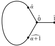
FIGURE 18. The subdivision complex for f .
