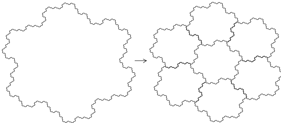
FIGURE 8. The subdivision of the tile type of the finite subdivision rule associated to the Lattès map with (a, b, c, d) = (2, -3, 1, 2) .
