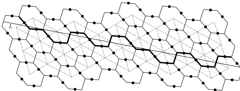
FIGURE 3. Constructing the edge path approximation of the line L .
