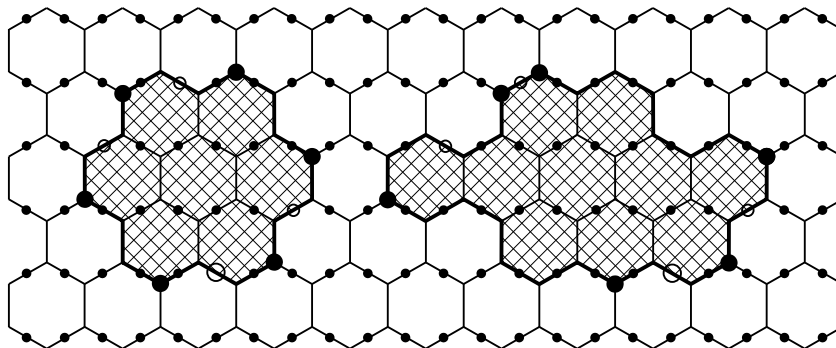
FIGURE 7. Fundamental domains for the cases in which (a, b, c, d) = (2, -3, 1, 2) with \beta = 0 and (a, b, c, d) = (2, -6, 1, 2) with \beta = 0 .
