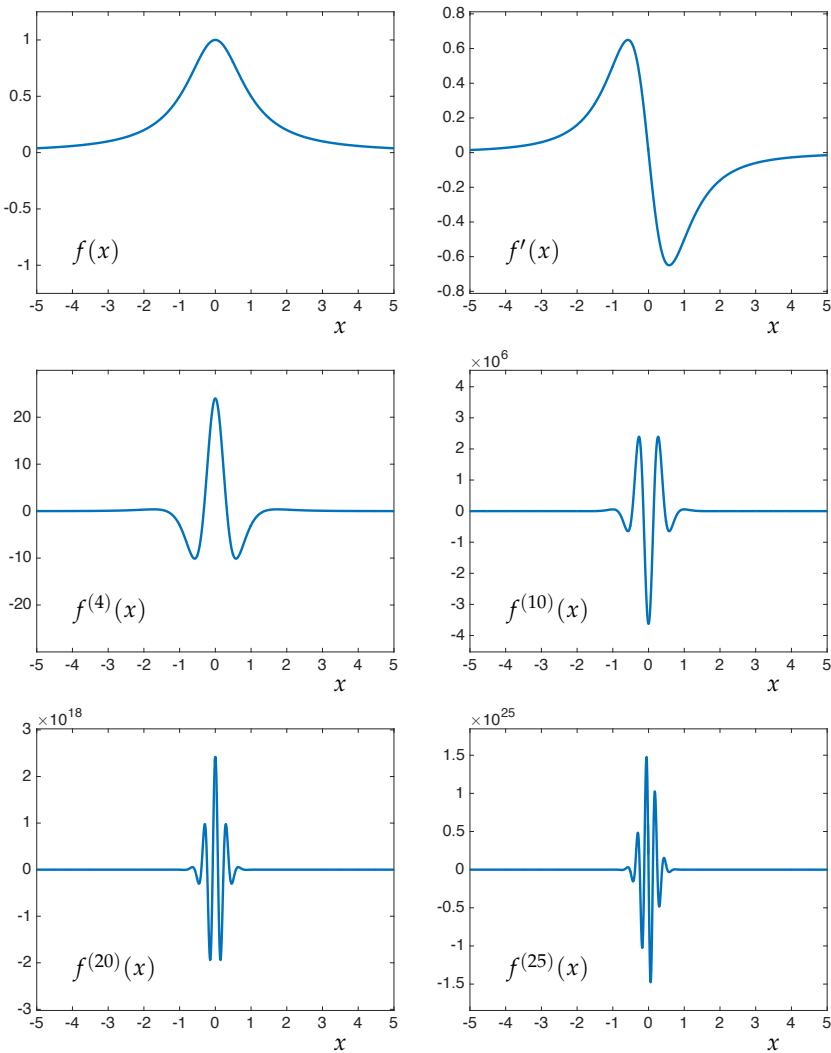
Figure 1.9: Runge's function
