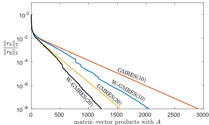
FIG. 11. GMRES(m) and W-GMRES(m) for a discretization of the Dirichlet Laplacian on the unit square. The eigenvectors are not localized, but weighting still accelerates convergence.
