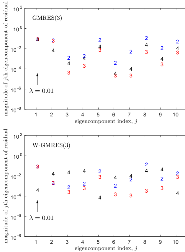
FIG. 4. Eigencomponents of the residual at the end of cycles \ell = 2, 3, and 4 for standard GMRES(3) (top) and W-GMRES(3) (bottom) applied to the matrix in Example 3.1. Cycle 4 of W-GMRES(3) reduces the eigencomponent corresponding to \lambda_1 = 0.01 by two orders of magnitude.
