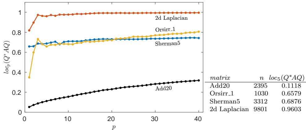
FIG. 12. Eigenvector localization measures loc_p(Q^*AQ) for the coefficient matrices transformed by the DCT matrix Q^* = \text{dct}(\text{eye}(\mathbf{n})) . The transformation reduces the localization of the Add20 eigenvectors, while significantly enhancing localization for the three other matrices.
