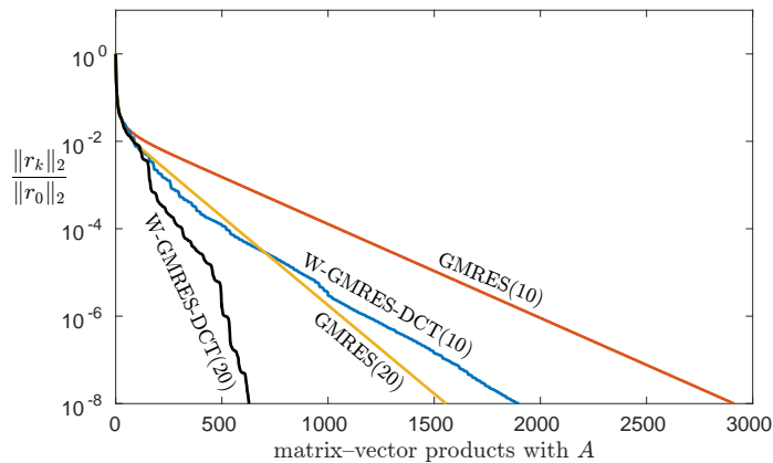
FIG. 14. GMRES(m) and W-GMRES-DCT(m) for the 2d Dirichlet Laplacian (Example 3.7). The DCT localizes the eigenvectors, improving the convergence of W-GMRES(m) in Figure 11.
