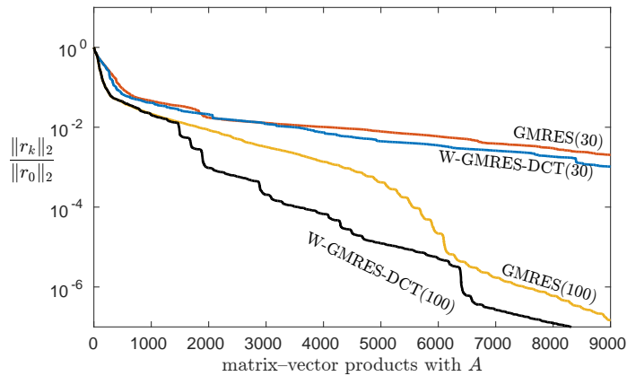
FIG. 13. GMRES(m) and W-GMRES-DCT(m) for the nonsymmetric Sherman5 matrix. The DCT helps to localize the eigenvectors, resulting in significantly better convergence than seen for W-GMRES(m) in the top plot of Figure 10.
