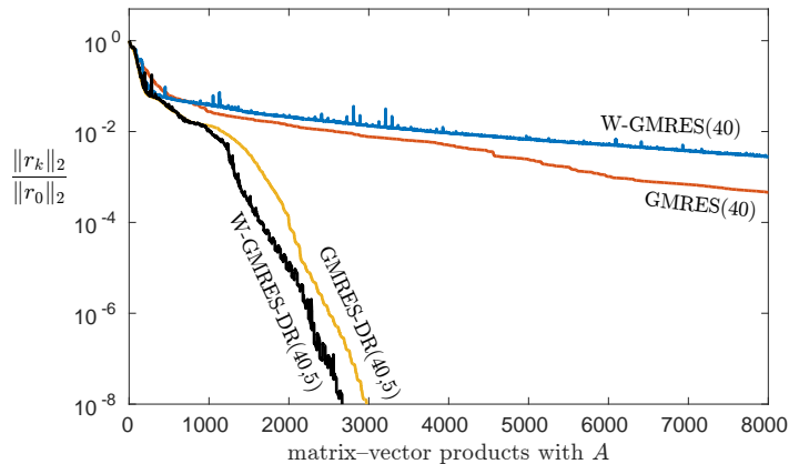
FIG. 17. Comparison of methods with and without weighting and deflation for Sherman5.
