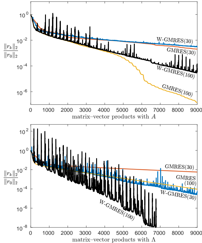
FIG. 10. GMRES(m) and W-GMRES(m) for the Sherman5 matrix. On the top, the methods are applied to Ax = b , and weighting slows convergence. On the bottom, the same methods are applied to \Lambda x = b , where \Lambda is diagonal with the same eigenvalues of A ; W-GMRES converges better. (The GMRES(100) curve is yellow. Color is available online only.) For both problems, taking m = 100 steps with each weighted inner product gives large growth in \|r_k\|_2 between restarts.
