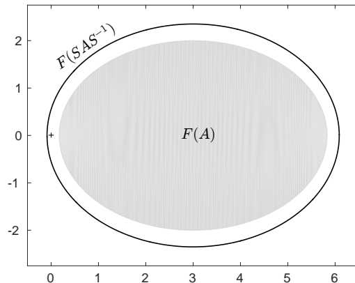
FIG. 8. The fields of values F(A) (gray region) and F(SAS^{-1}) (boundary is a black line) in \mathbb{C} for A and r_0 in (8); the cross (+) marks the origin. Since 0 \notin F(A) , GMRES( m ) converges for any r_0 ; however, 0 \in F(SAS^{-1}) and (Sr_0)^*(SAS^{-1})(Sr_0) = 0 , so W-GMRES(1) completely stagnates.
